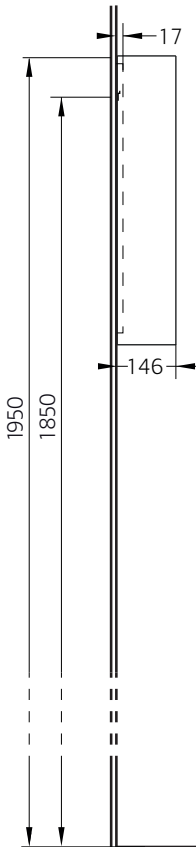
SIDE
