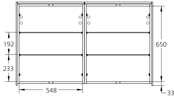
INSIDE
